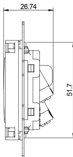
Product dimensions (mm, for reference)
