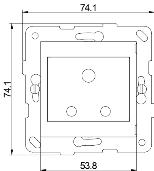
Product dimensions (mm, for reference)
